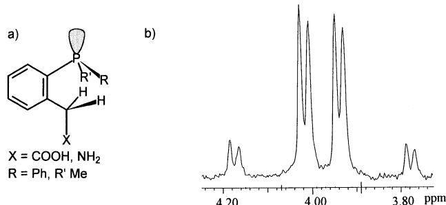
Figure 2. (a) Conformation of the \text{CH}_2\text{-X} group in 12 and 17 ; (b) ^1\text{H} -NMR spectrum ( \text{CH}_2 -part) of 17
