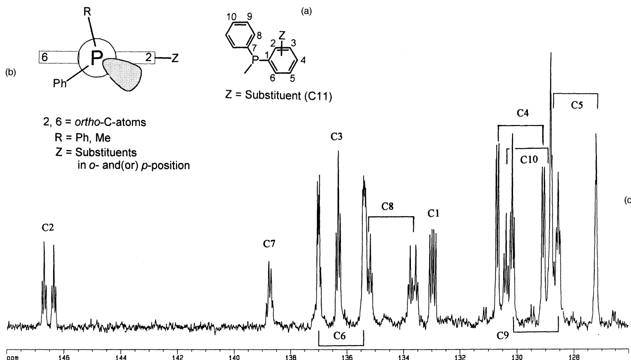
Figure 1. (a) Numbering scheme for the carbon atoms in mono- and disubstituted aromatic phosphanes; (b) conformation of the Ph(R)P-group with respect to the plane of the substituted aromatic ring; (c) ^{13}\text{C} -NMR spectrum of 8
