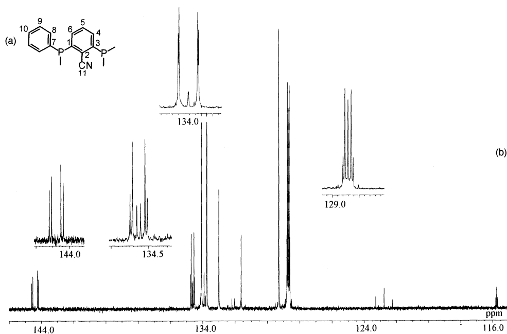
Figure 3. (a) Numbering scheme for the carbon atoms in 23 ; (b) ^{13}\text{C}\{^1\text{H}\} -NMR spectrum of 23
